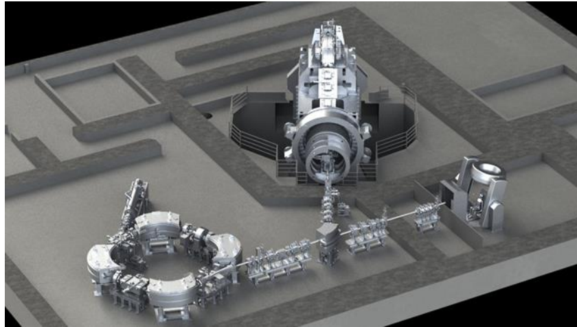
Proton therapy equipment combined with Hitachi’s 360° rotating gantry and Leo’s upright system
